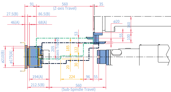
TRIPLE ID HOLDER
