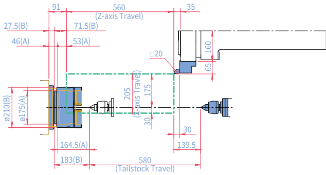
STRAIGHT MILLING HOLDER
