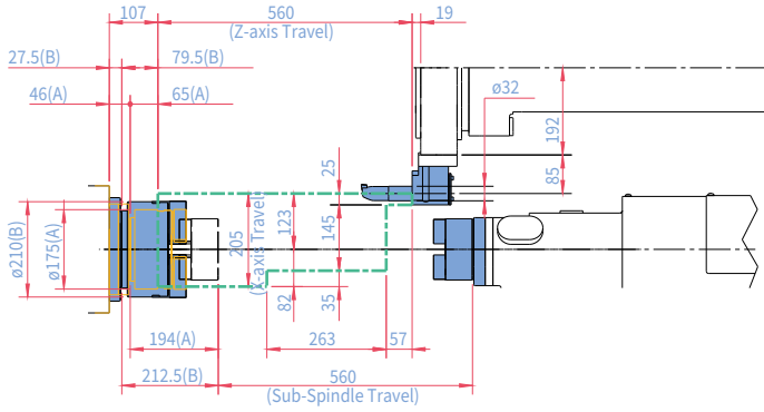
FACE TOOL HOLDER
