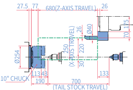
ID HOLDER
