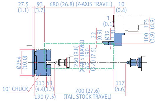
FACE HOLDER
