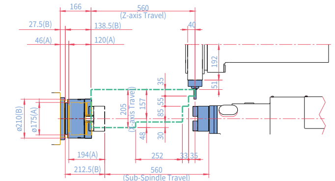
STRAIGHT MILLING HOLDER
