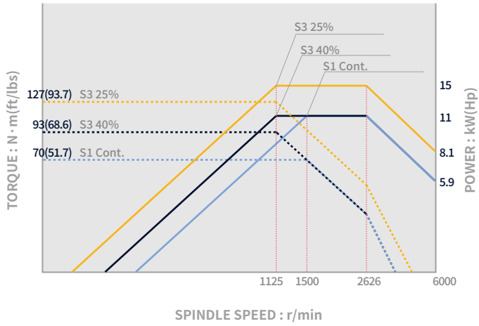
Main Spindle_Lynx 2100LYA / LSYA
