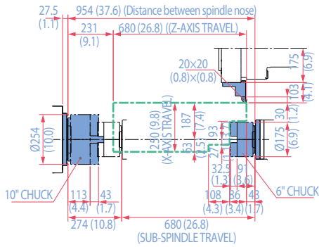
DOUBLE OD-R HOLDER
