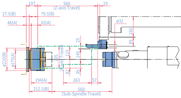
ID HOLDER
