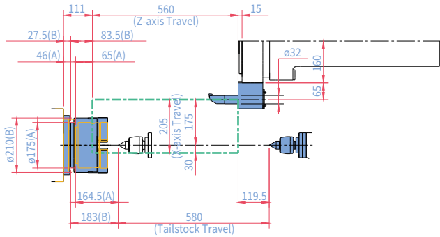
ID HOLDER
