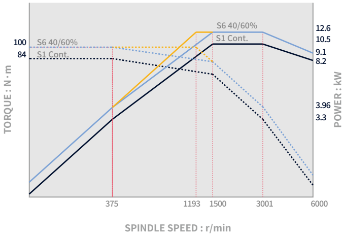
Main Spindle_Lynx 2100LYA / LSYA
