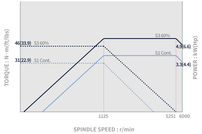
Sub-Spindle_Lynx 2100LSYA / LSYB
