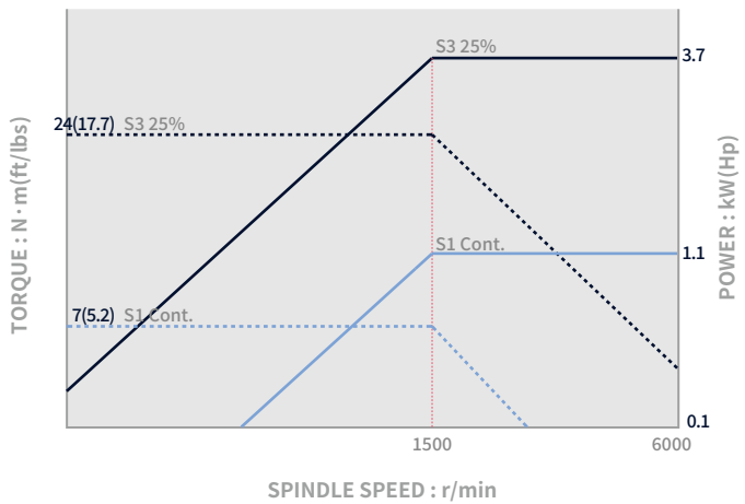
Rotary Tool_Lynx 2100LY / LSY
