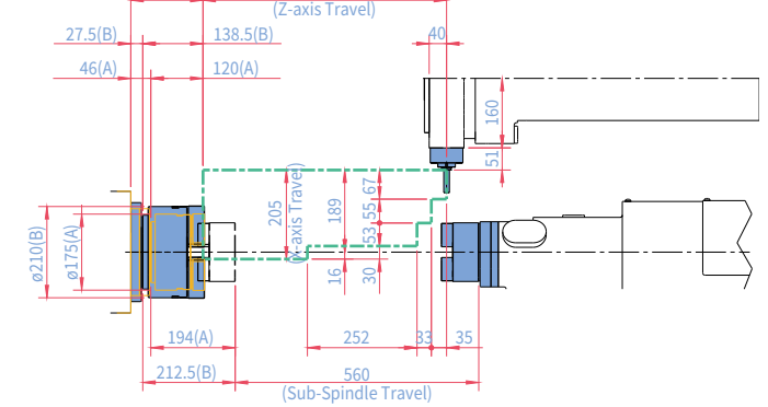
STRAIGHT MILLING HOLDER
